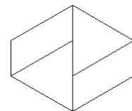
HATE 50 100
